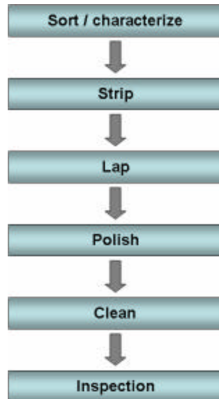
Figure 1. Outline of the wafer reclaim indicating the key processing steps.
